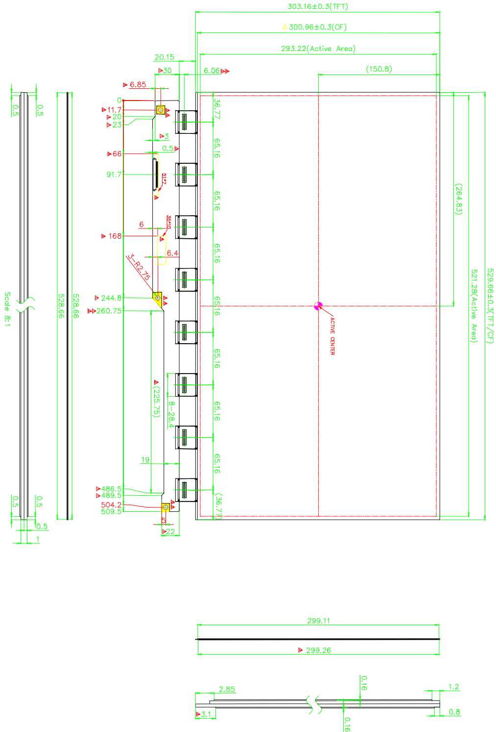
Figure 5. TFT-LCD Open Cell Outline Dimensions (Front view)
