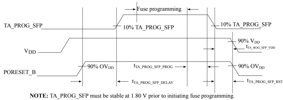
Figure 10. TA_PROG_SFP timing diagram
