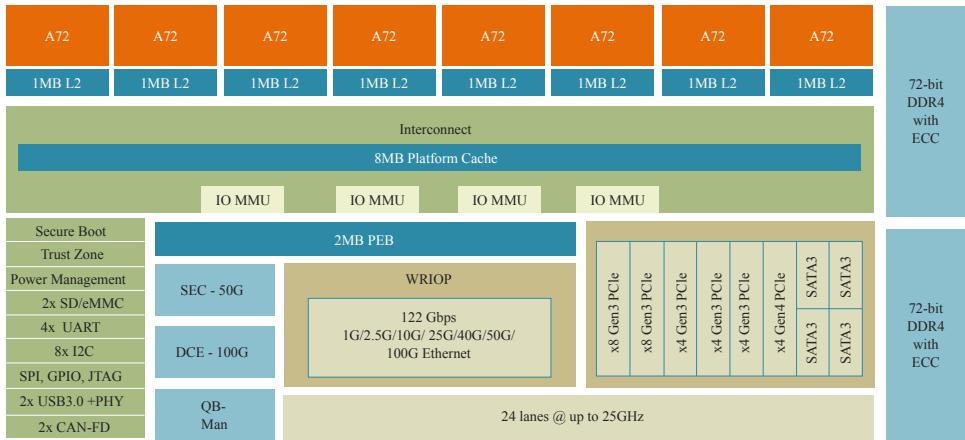
Figure 3. LX2080A Block diagram
