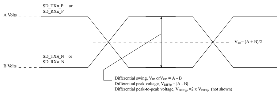
Figure 45. Differential voltage definitions for transmitter or receiver
