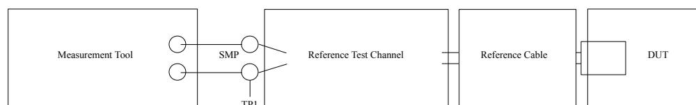
Figure 43. Transmit normative setup
