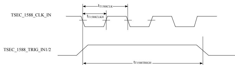
Figure 27. IEEE 1588 input AC timing
