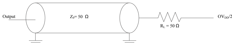
Figure 32. AC test load for the JTAG interface
