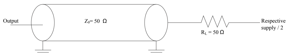
Figure 29. Flextimer AC test load
