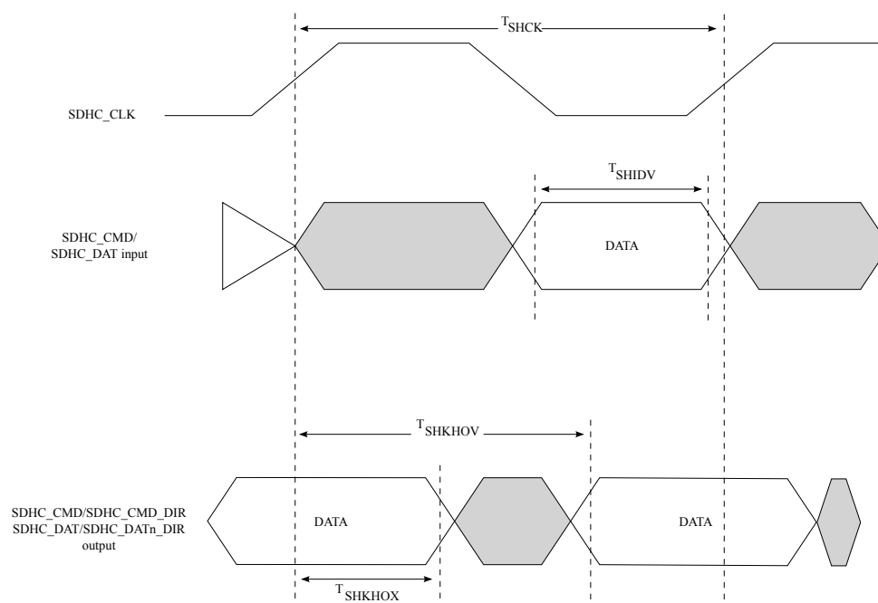
Figure 16. eSDHC SDR104/HS200 mode timing diagram
