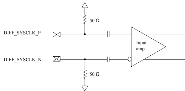
Figure 11. DIFF_SYSCLK_P/DIFF_SYSCLK_N receiver
