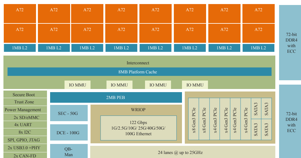
Figure 1. LX2160A Block diagram
