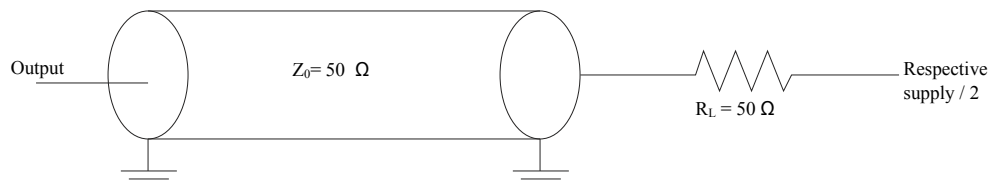
Figure 28. GPIO AC test load
