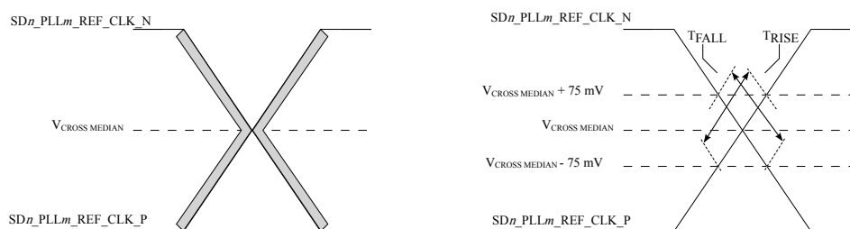
Figure 51. Single-ended measurement points for rise and fall time matching
