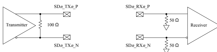
Figure 52. SerDes transmitter and receiver reference circuits
