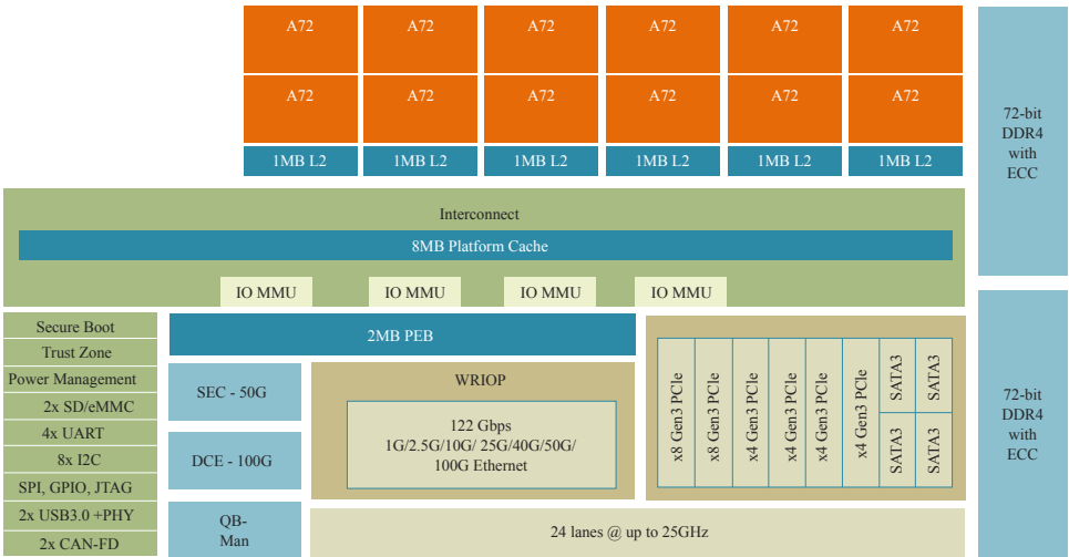
Figure 2. LX2120A Block diagram
