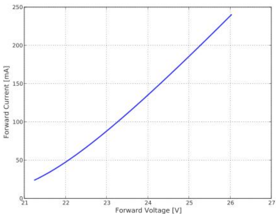
Figure4. Typical forward current VS forward voltage
