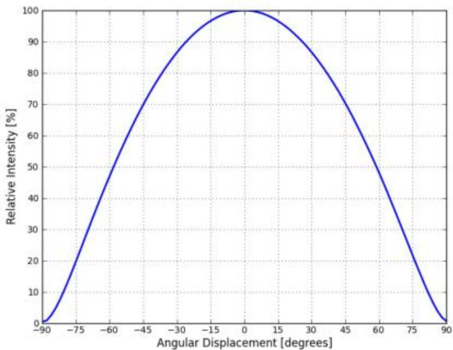
Figure7.Typical radiation patten
