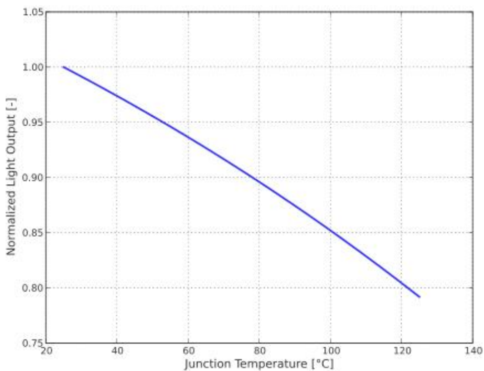
Figure6. Typical normalized light output vs Junction temperature
