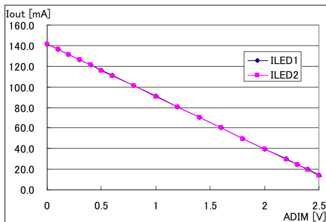
Fig. 5-3 Current Amplitude dimming characteristics(ADIM vs Iout)
