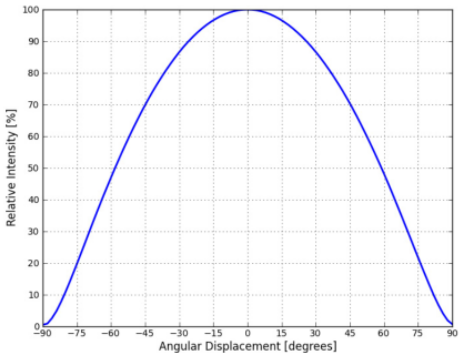
Figure7.Typical radiation patten
