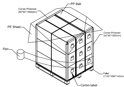
Figure. 6-2 Packing method
