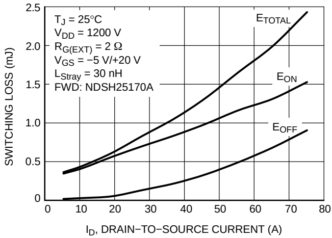
Figure 7. Switching Loss vs. Drain-to-Source Current ( 25^\circ\text{C} )
