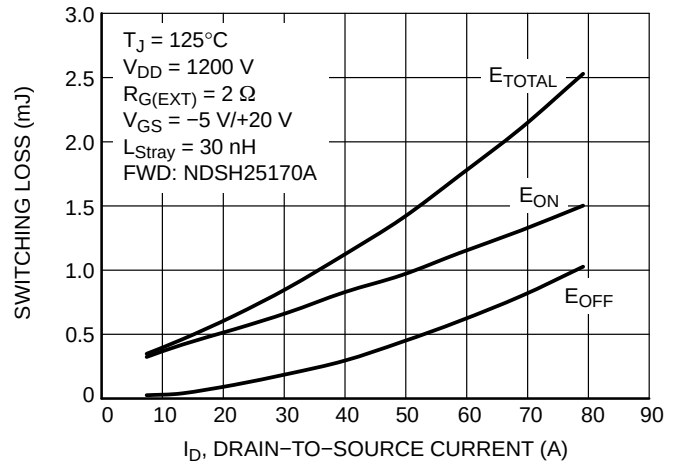
Figure 8. Switching Loss vs. Drain-to-Source Current ( 125^\circ\text{C} )
