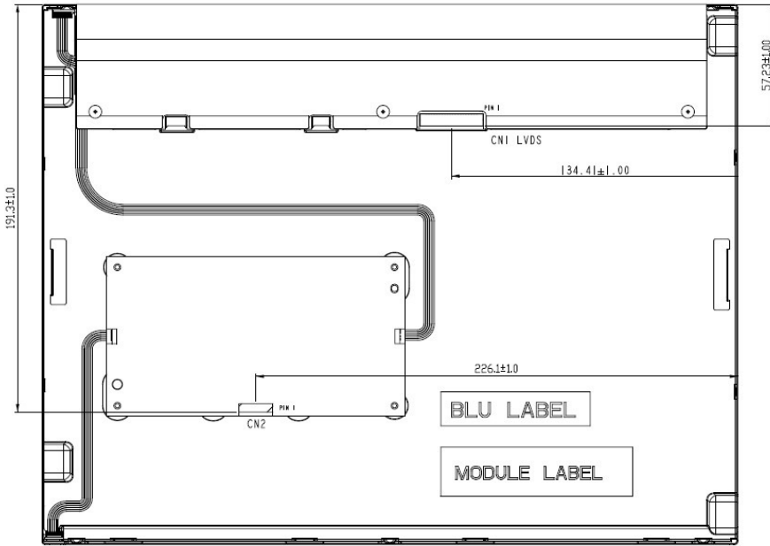
LVDS (CN1):
