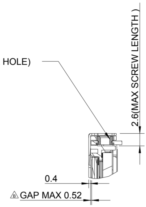
SECTION USER_HOLE-USER_HOLE SCALE 2:1
