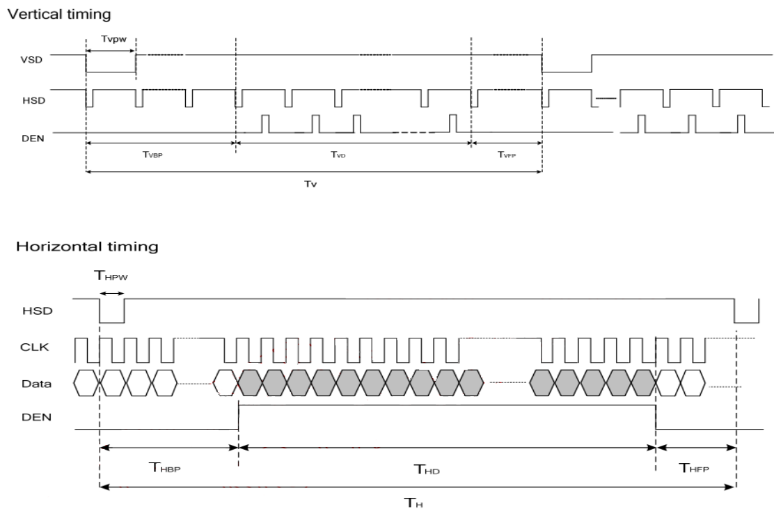
Figure 6.1.1 Clock and Data Input Timing Diagram
