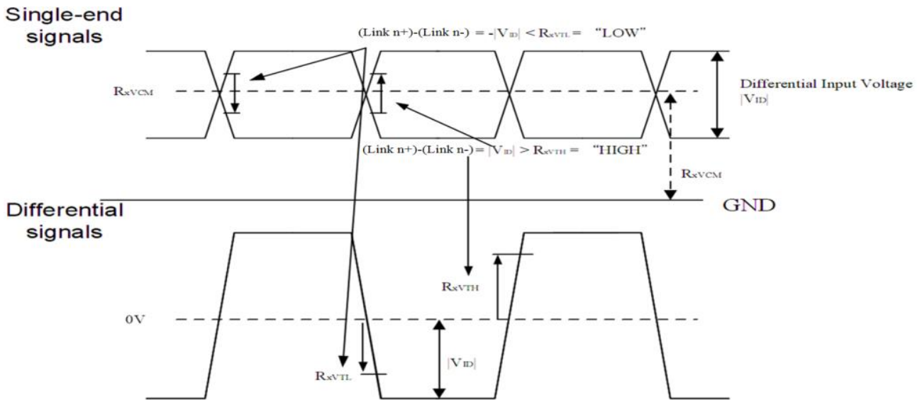
Figure 5.5.1 LVDS DC Characteristics
