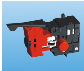
HT1010 Series 防塵交流扳機調速開關
