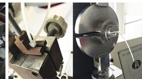
▶ 插入力测试、拉伸强度试验 Insertion force testing and Tensile strength testing
