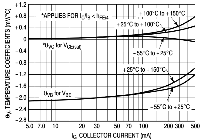
Figure 4. Temperature Coefficients
