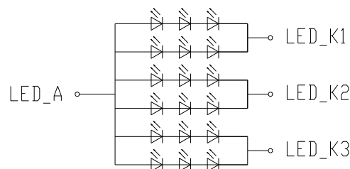
LED circuit
