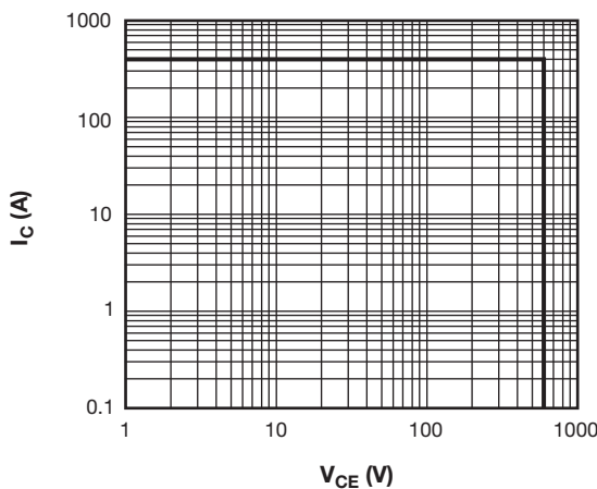
Fig. 15 - Reverse BIAS SOA, T_J = 150^{\circ}\text{C} , V_{GE} = 15\text{V}
