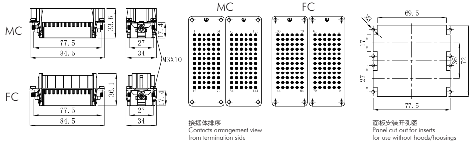
Dimensions mm
