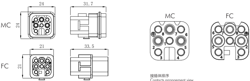
接插体排序 Contacts arrangement view from termination side
