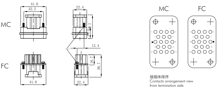
Dimensions mm
