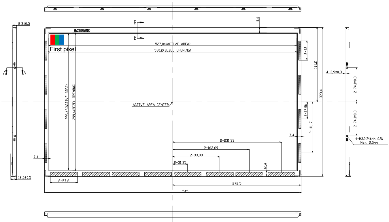
Figure 5. TFT-LCD Module Outline Dimensions (Front view)
