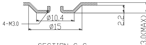
SECTION C-C SCALE 5/1
