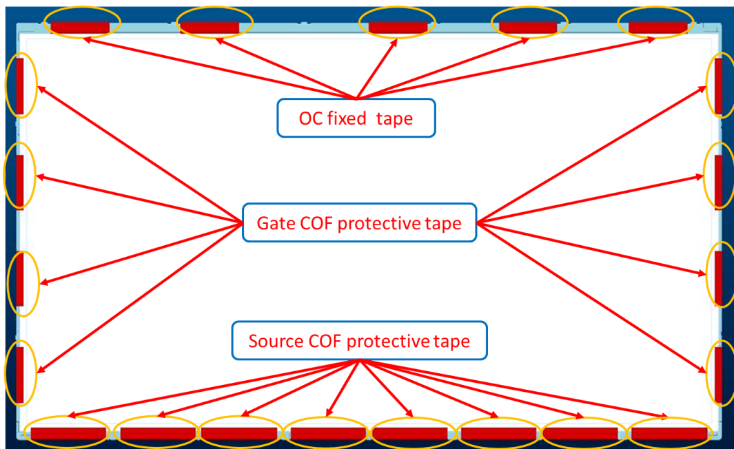
Figure 8. Paste position
