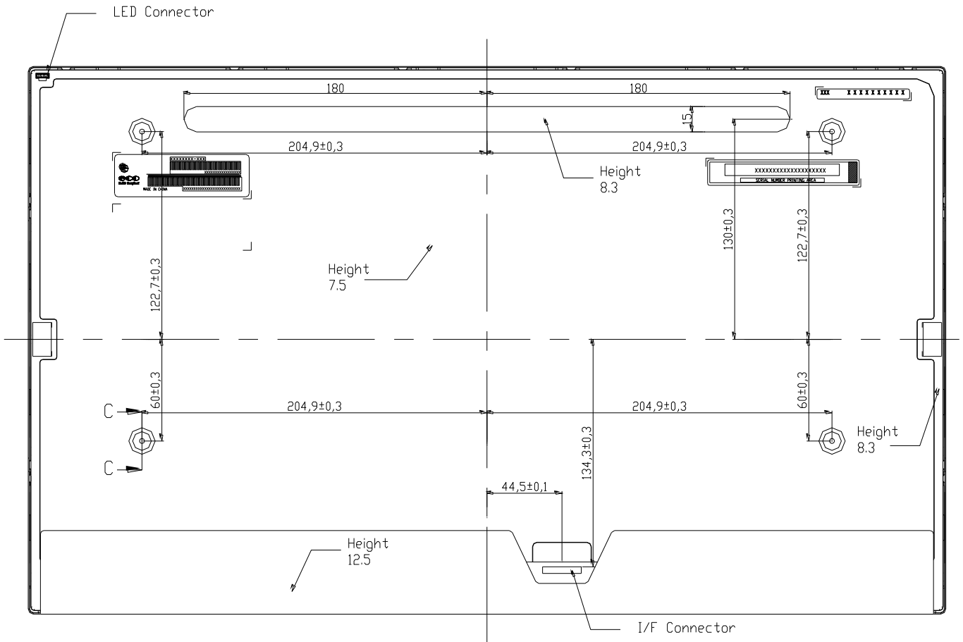
Figure 6. TFT-LCD Module Outline Dimensions (Rear view)
