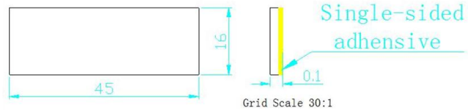
Figure 8. Paste position
