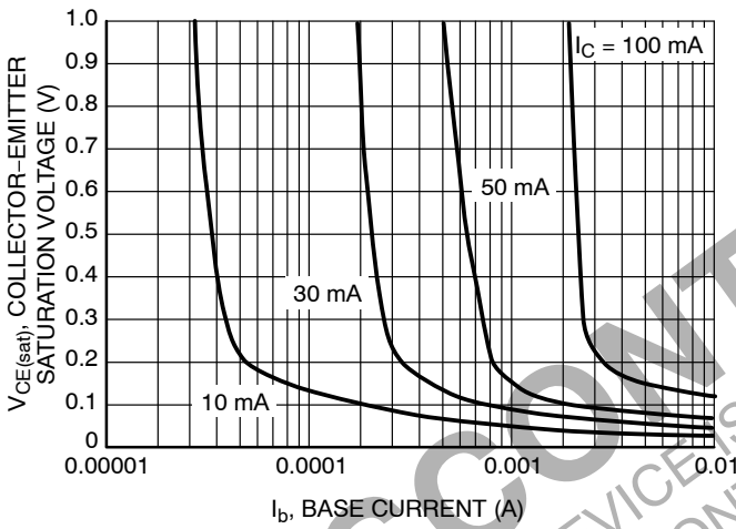
Figure 5. Saturation Region
