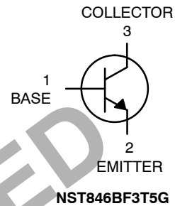
SOT-1123 CASE 524AA STYLE 1 (Rotated 90° Clockwise)
