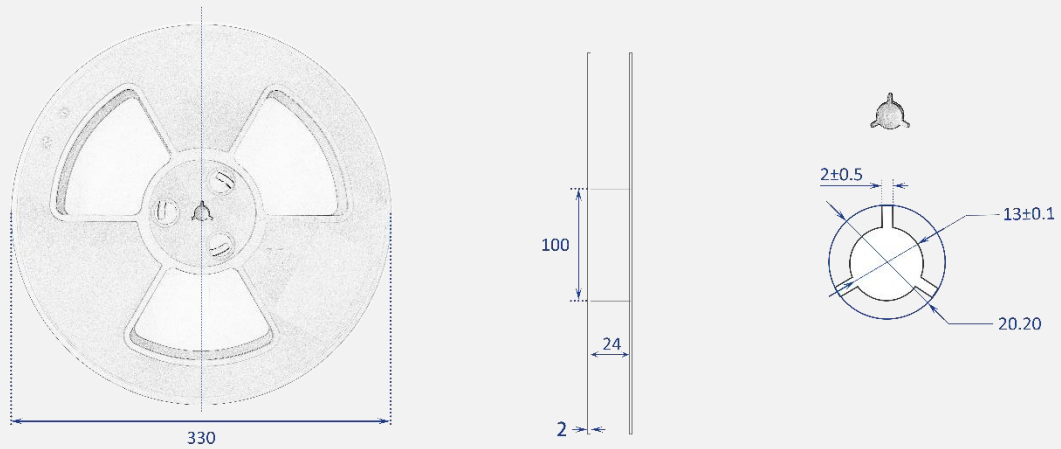
Figure 10 Reel dimensions
