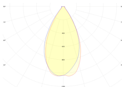
GSLED 5050.V6X.20 FWHM = 54°×55°, \eta = 91,7 %
