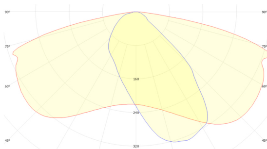
GSLED 5050.V6B.50 FWHM = 157°×58°, \eta = 94,9 %
