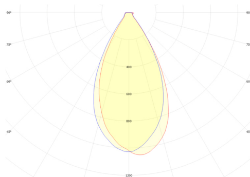
GSLED 5050.V6X.41 FWHM = 51°×55°, \eta = 90,2 %
