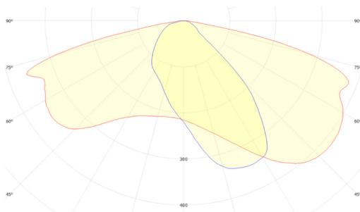
GSLED 5050.V6X.40 FWHM = 154°×57°, \eta = 96,8 %
