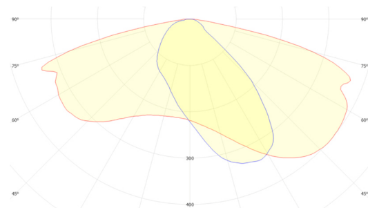
GSLED 5050.V6X.41 FWHM = 154°×58°, \eta = 95,2 %
