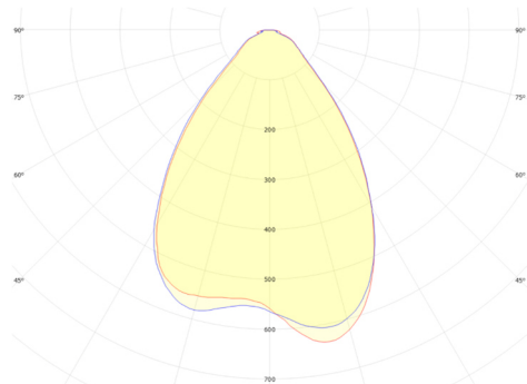
GSLED 5050.V6X.40 FWHM = 72°, \eta = 94,3 %
