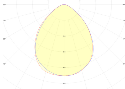
Refond RF-Q50SA40B FWHM = 89°, \eta = 92,1 %
