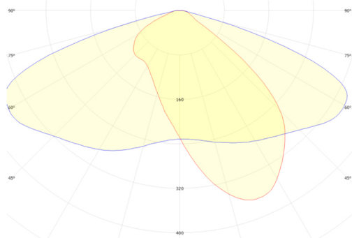
Refond RF-Q50SA40B FWHM = 145^{\circ} \times 58^{\circ} , \eta = 92,7\%
