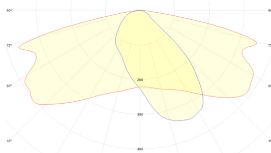
GSLED 5050.V6X.20 FWHM = 156°×59°, \eta = 97,2 %
