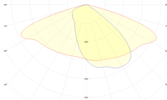
Samsung LH351C FWHM = 145^\circ \times 67^\circ , \eta = 98,0\%
