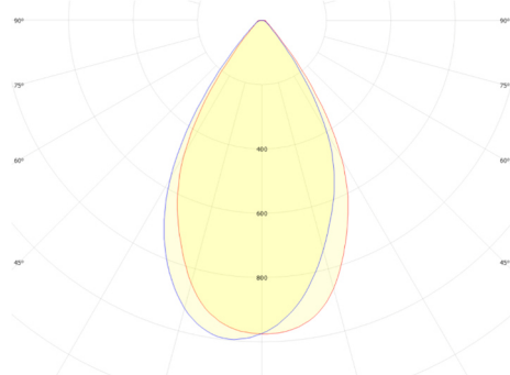
Refond RF-Q50SA40B FWHM = 60°, \eta = 93,8 \%
