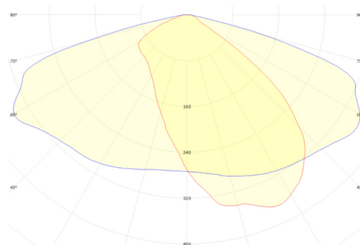
GSLED 5050.V6X.20 FWHM = 149°×67°, \eta = 95,0 %
