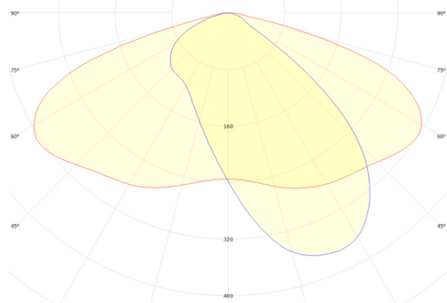
Refond RF-Q50SA40B FWHM = 147^\circ \times 59^\circ , \eta = 95,5\%
