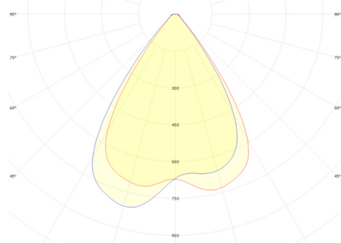
Samsung LH351C FWHM = 70°, \eta = 95,0 \%
