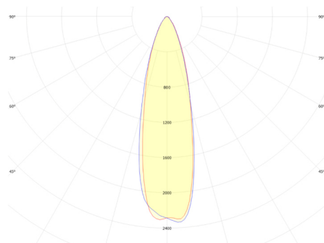
GSLED 5050.V6B.50 FWHM = 27°, \eta = 93,2 %
