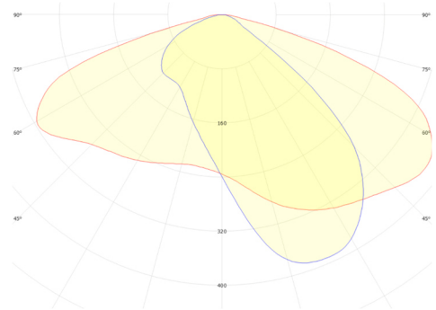
GSLED 5050.V6X.40 FWHM = 144°×57°, \eta = 94,7 %
