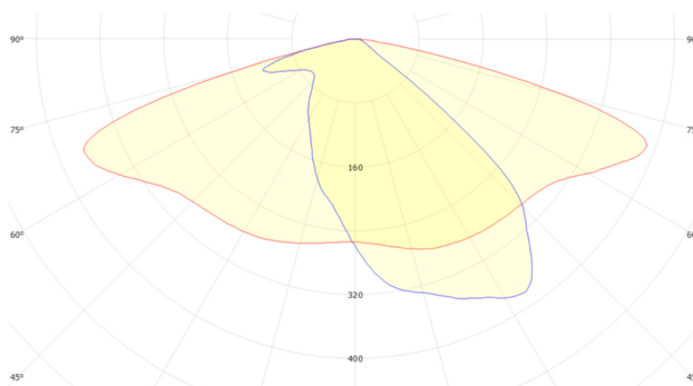
GSLED 5050.V6B.50 FWHM = 151°×63°, \eta = 96,5 %
