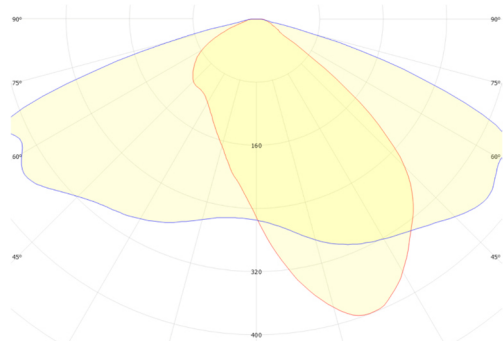
Seoul STW0L8PA FWHM = 144^{\circ} \times 58^{\circ} , \eta = 93,1\%
