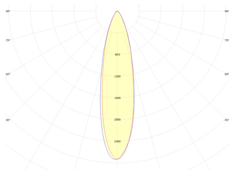
Клевер CLP-5050F5A FWHM = 24°, \eta = 95,0 %
