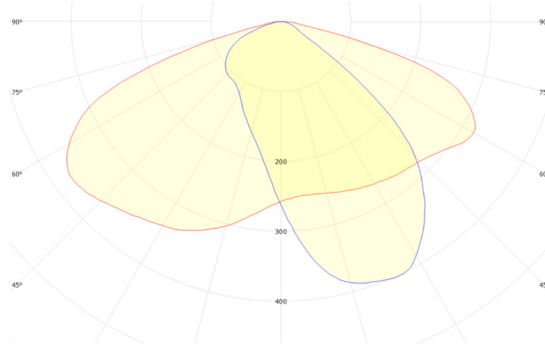
GSLED 5050.V6X.41 FWHM = 145°×57°, \eta = 94,4 %
