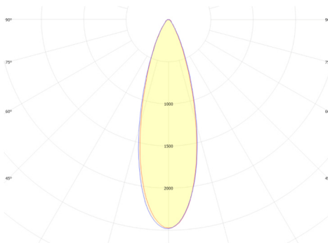
GSLED 5050.V6X.41 FWHM = 30°, \eta = 91,0 %
