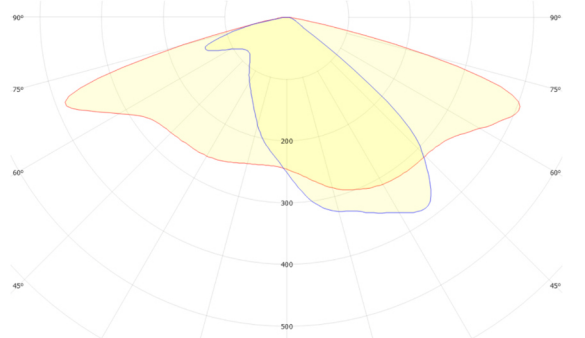
GSLED 5050.V6X.41 FWHM = 150°×64°, \eta = 97,9 %
