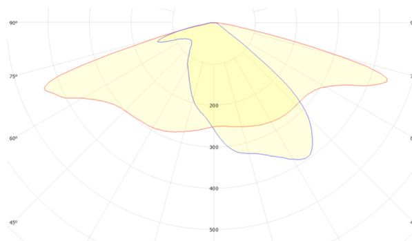
GSLED 5050.V6X.20 FWHM = 150°×64°, \eta = 98,5 %
