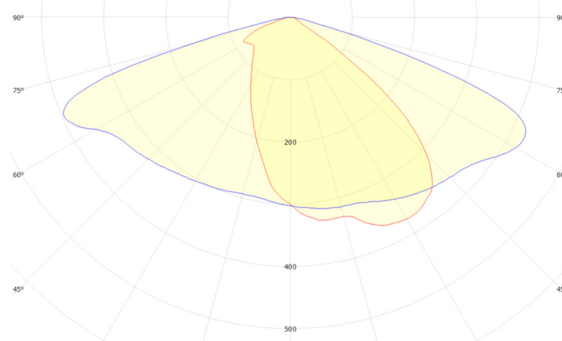
Samsung LH351C FWHM = 146^{\circ} \times 70^{\circ} , \eta = 96,1\%
