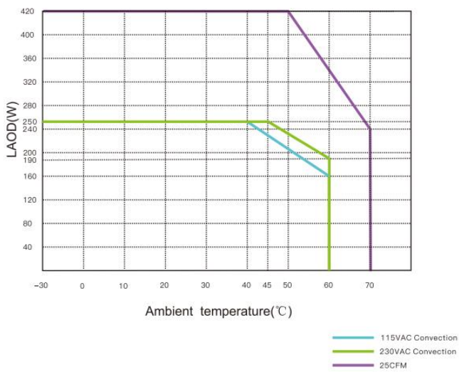
Derating curve
