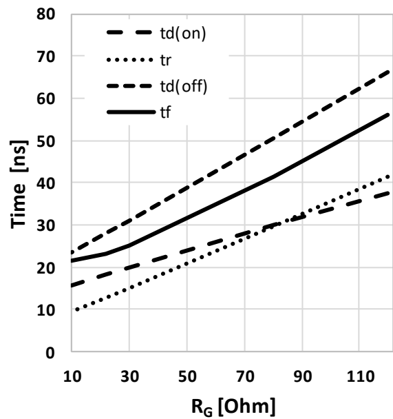
Figure 14 Typical switching times as a function of gate resistor ( t = f(R_{G,ext}), V_{DD} = 1000V, V_{GS} = 0V/12V, I_D = 1.5A, T_{vj} = 175^\circ C, ind. load, test circuit in Fig. E, diode: body diode at V_{GS} = 0V )
