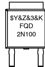
DPAK3 (TO-252 3 LD) CASE 369AS
