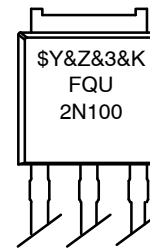
DPAK3 (IPAK) CASE 369AR
