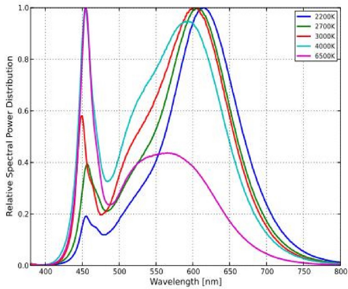
Figure2. Typical Color Spectrum for 80CRI
