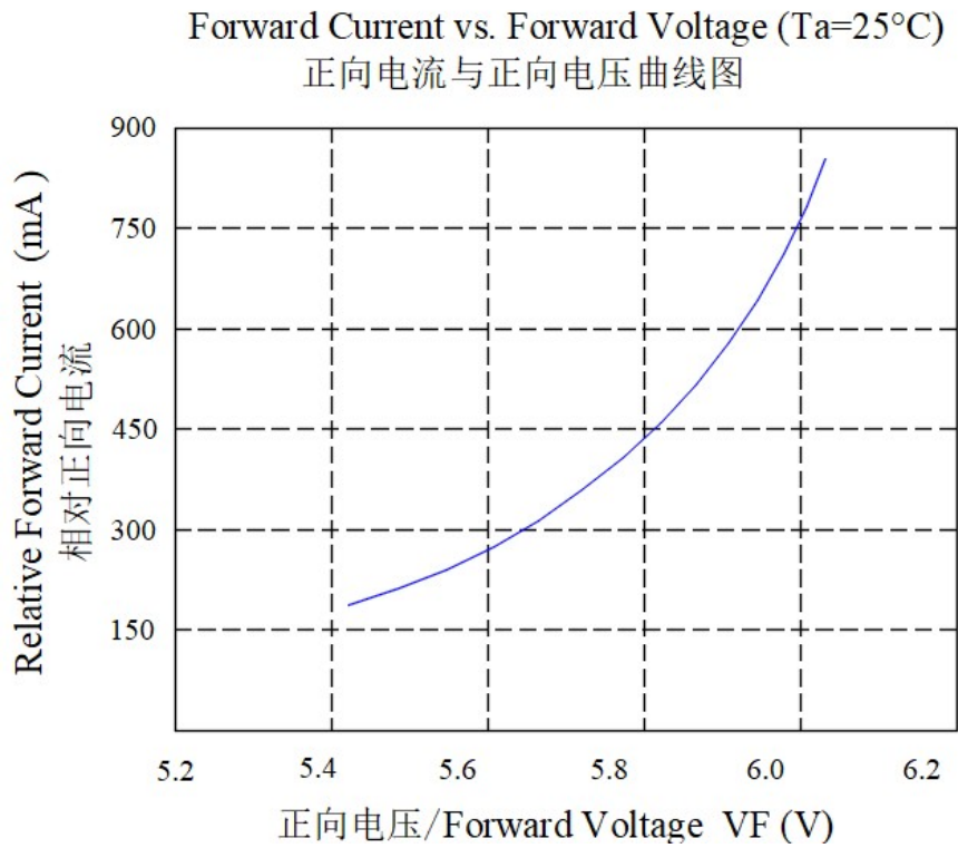
Figure3. Typical forward current VS forward voltage
