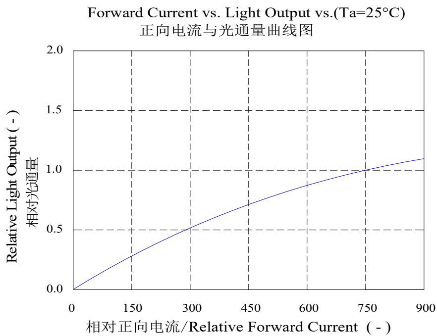
Figure4. Typical normalized light output vs. forward current
