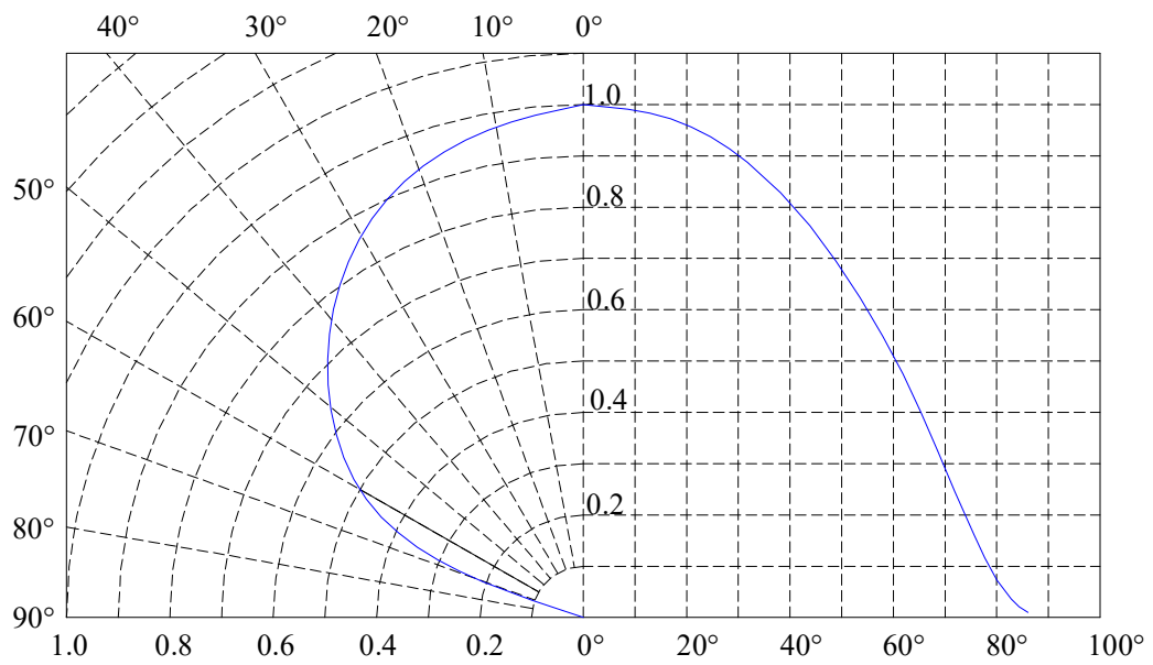
Figure6. Radiation Characteristics
