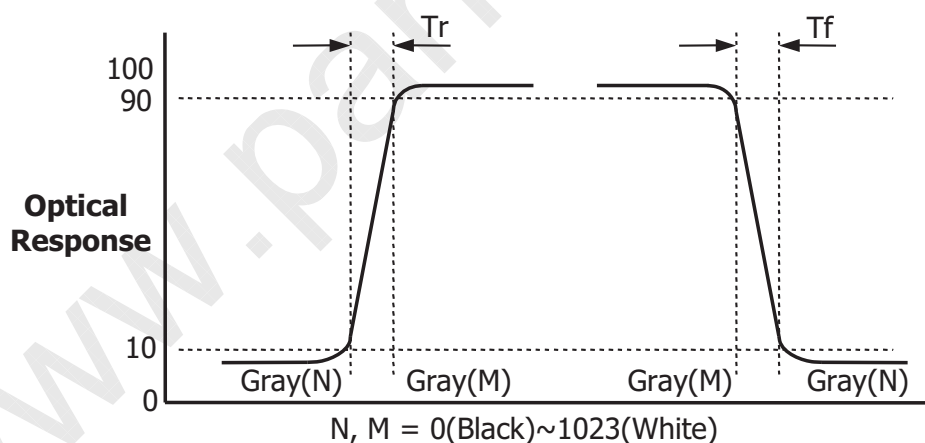
FIG.4-3 Response Time
