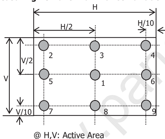
FIG.4-2 Measure Point for Luminance
