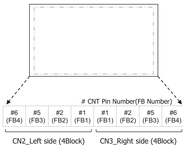
[ Front view of LCM ]
