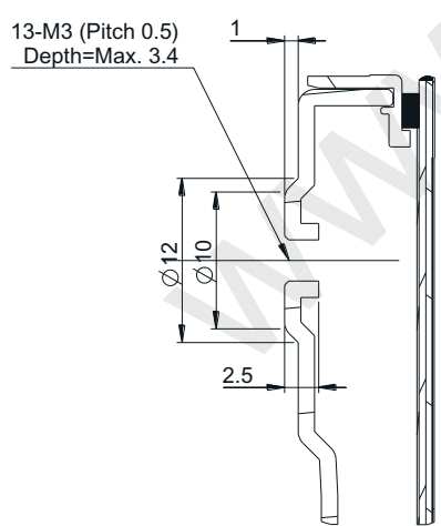
SECTION A-A SCALE 2/1
