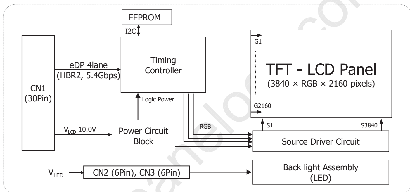
FIG.1 Block Diagram
