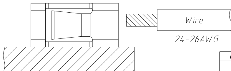
Assembly Layout
