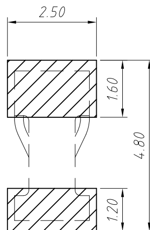
Board Layout
