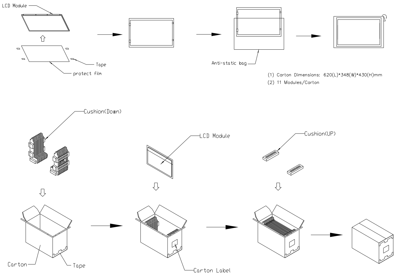
Figure. 7-1 Packing method
