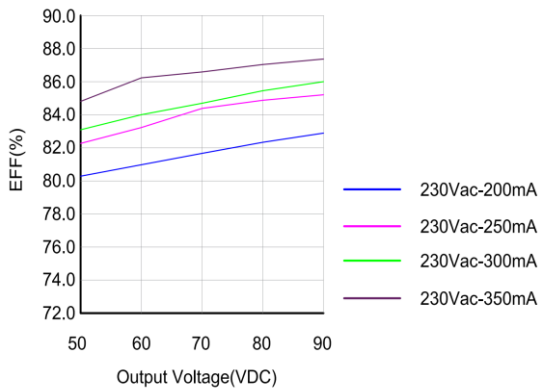
Efficiency VS.Load
