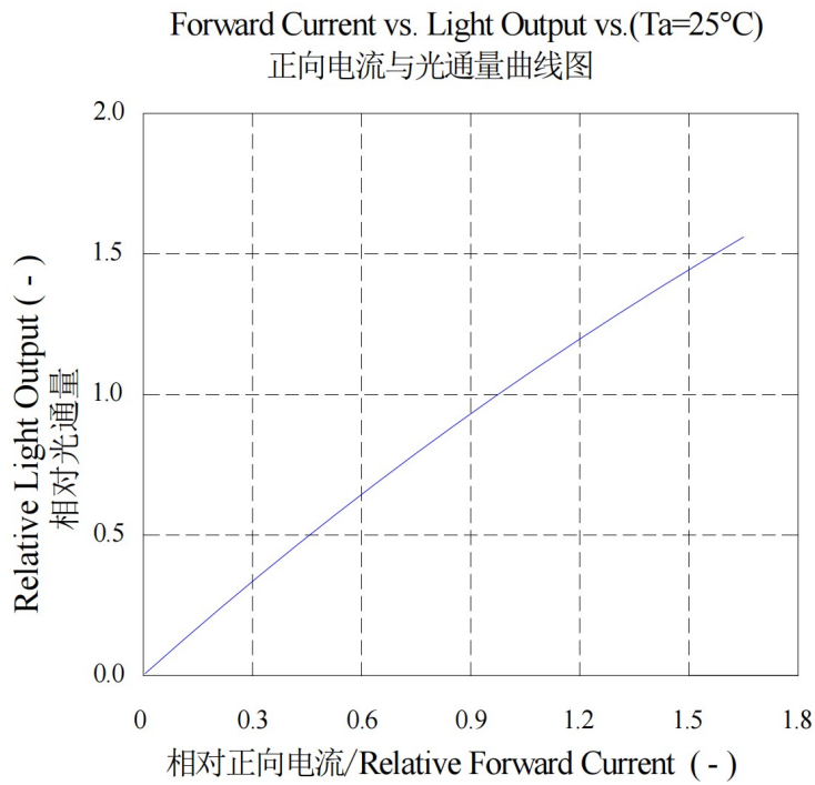
Figure4. Typical normalized light output vs. forward current
