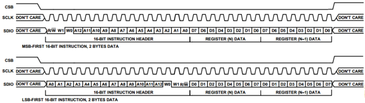
MSB First and LSB First Instruction and Data Phases
