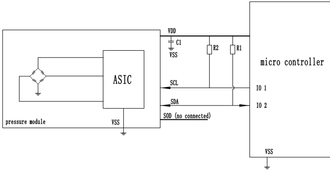
I 2 C Application Circuit
