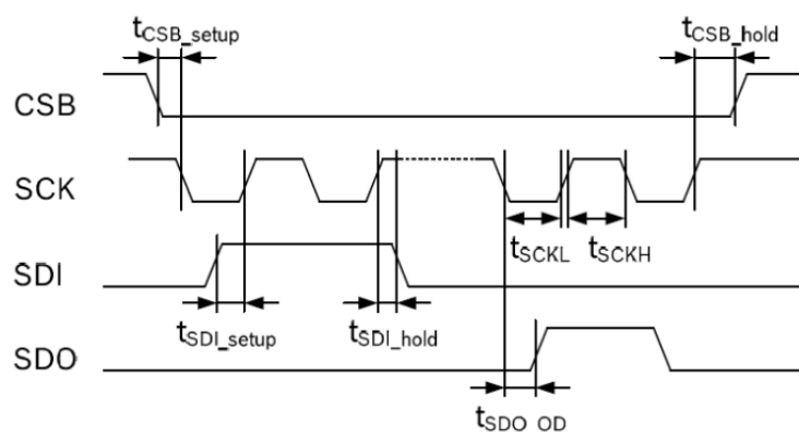
SPI timing diagram
