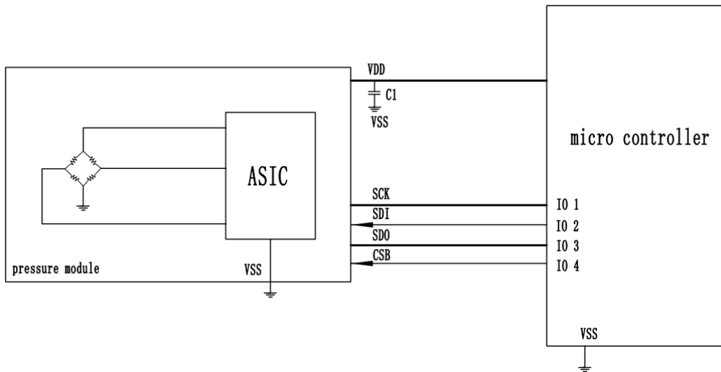
SPI Application Circuit
