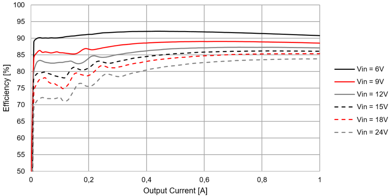
173010335 V_{OUT} = 3.3V , f_{SW} = 520kHz , T_A = 25^\circ C
