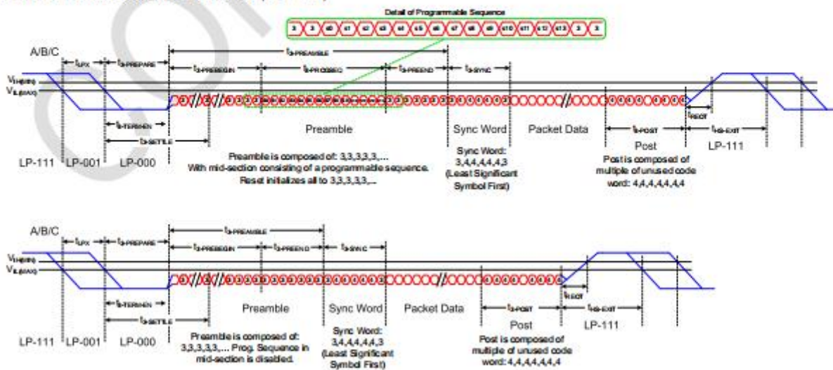
HS Data Transmission in Burst (C-PHY)
