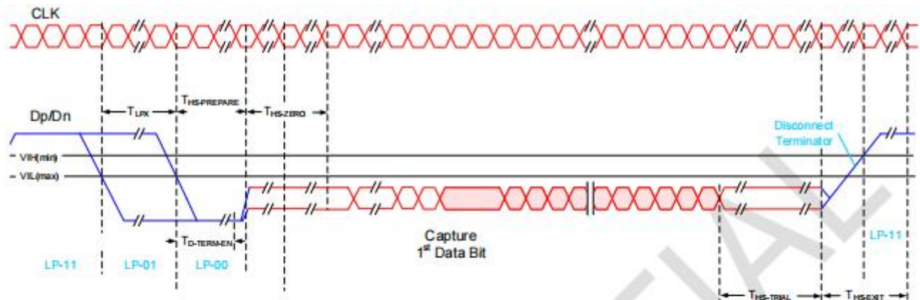
HS clock transmission (D-PHY)
