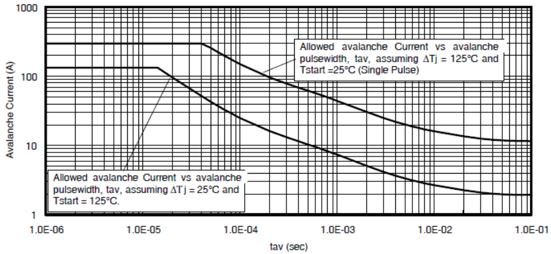
Fig 14. Typical Avalanch Current vs. Pulsewidth
