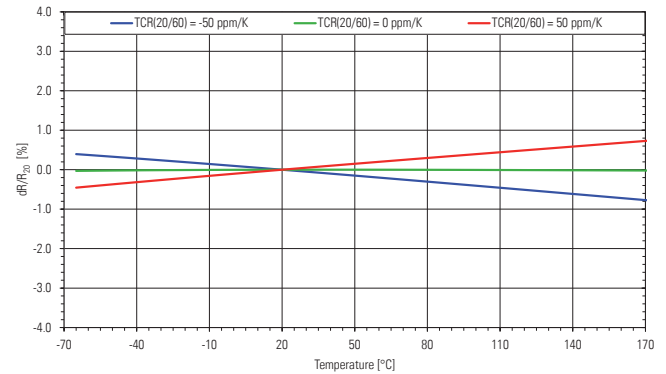
Temperature dependence of the electrical resistance of ISAOHM® resistors. Example: BVT-I-R002
