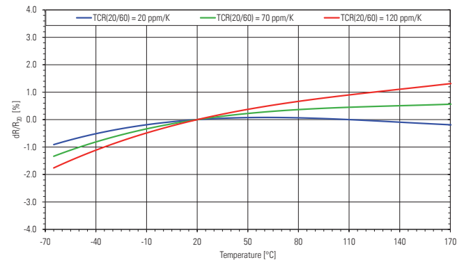
Temperature dependence of the electrical resistance of MANGANIN® resistors. Example: BVT-M-R0005
