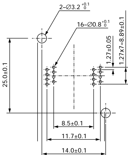
16 pins (SOP) IC51-0162-1025
