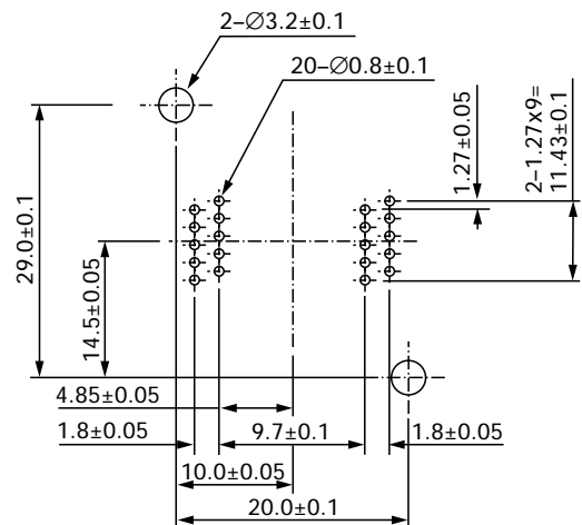
20 pins (SOP) IC51-334.KS-13574
