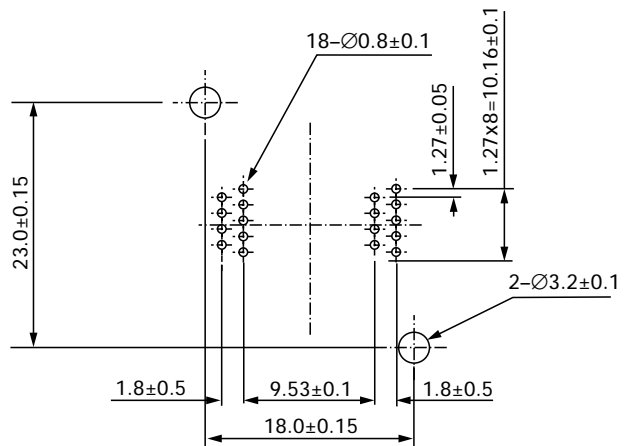
18 pins (SOP) IC51-0347.KS-6768
