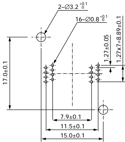
16 pins (SOP) IC51-0162-902-2
