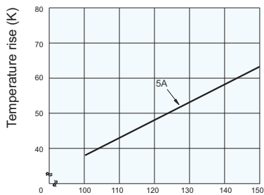
COIL TEMPERATURE RISE
