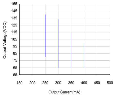
Operating window
