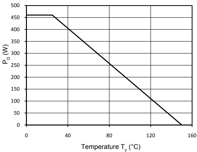
Figure 9. Power Dissipation
