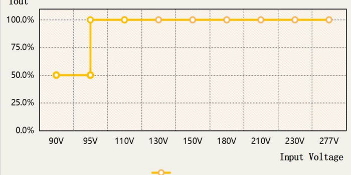
INPUT VOLTAGE VS OUTPUT Current 输入电压 VS 输出电流
